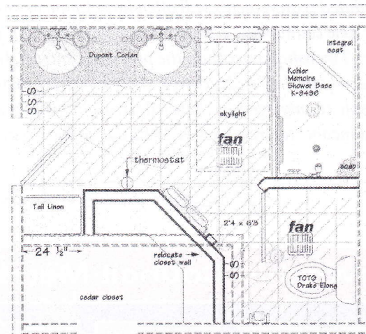
NEW FLOOR PLAN
